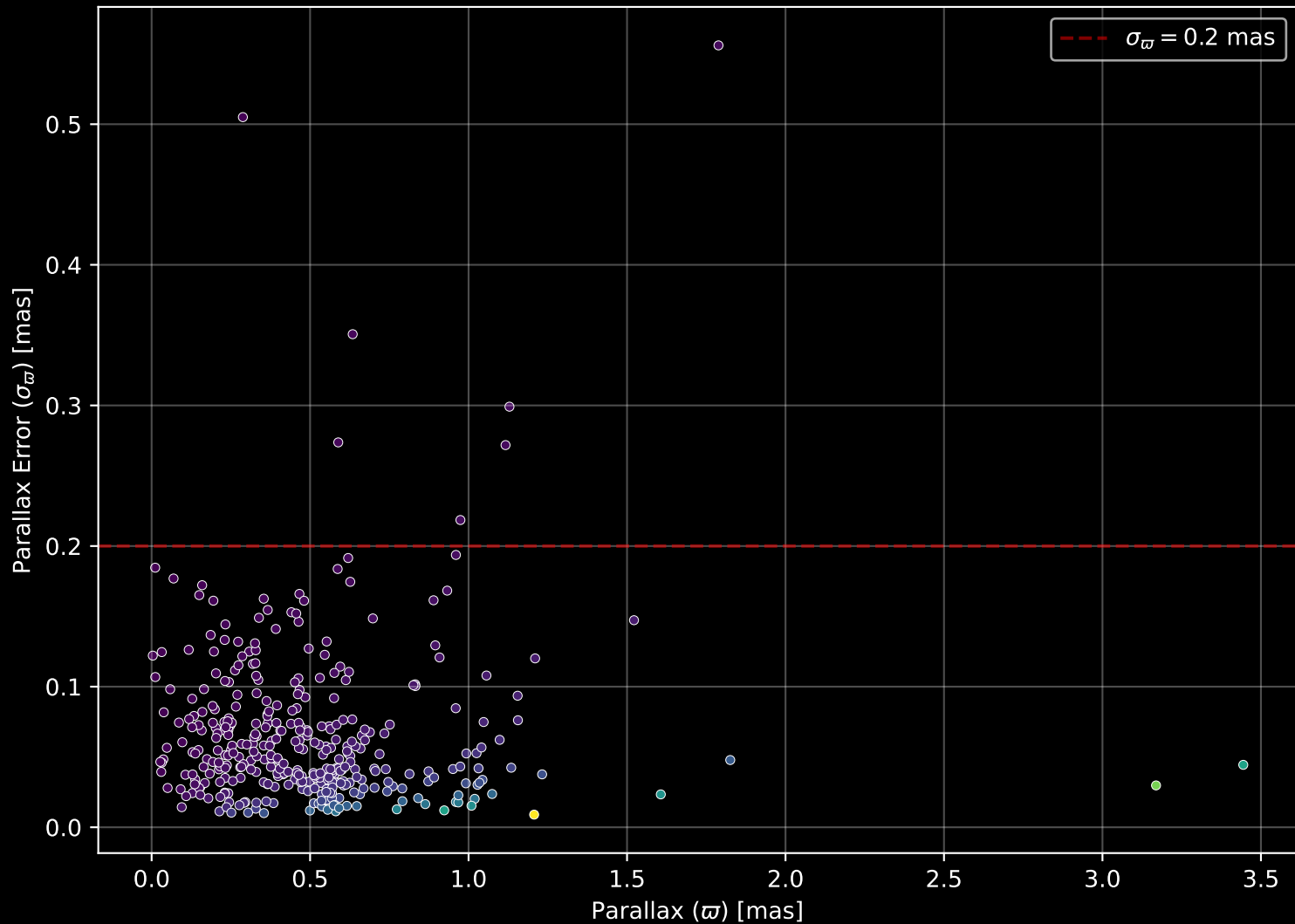
APOGEE DR17 Field: [CygnusX_S_btx] Parallax Quality (n= 372)
