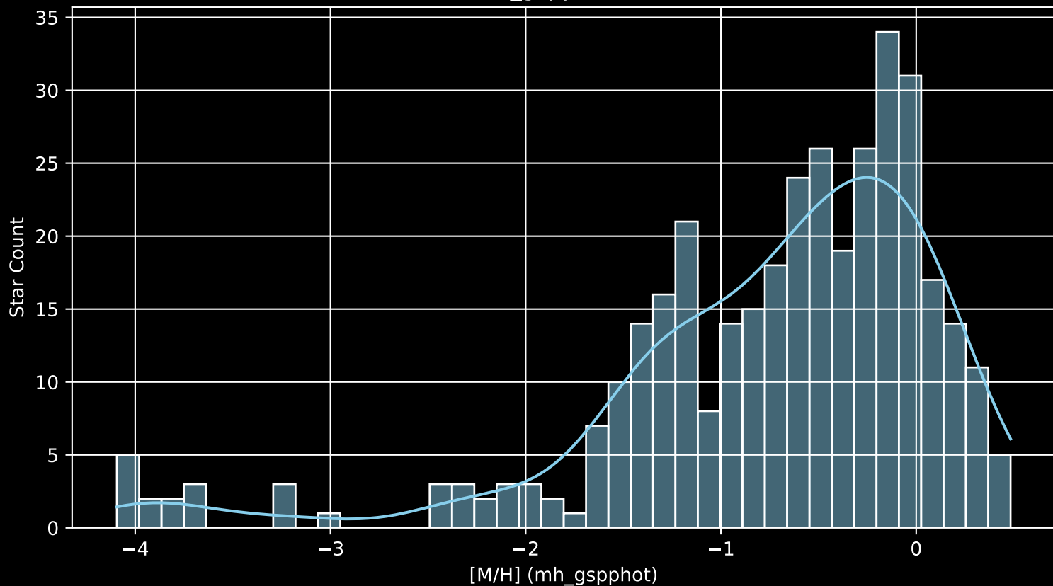
APOGEE DR17 Field: [CygnusX_S_btx [M/H] (mh_gspphot) (n= 363)
