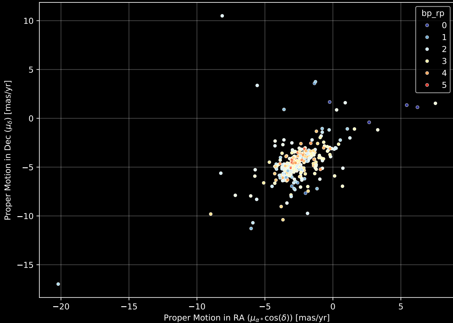
APOGEE DR17 Field: [CygnusX_S_btx] Proper Motion Diagram (n= 372)
