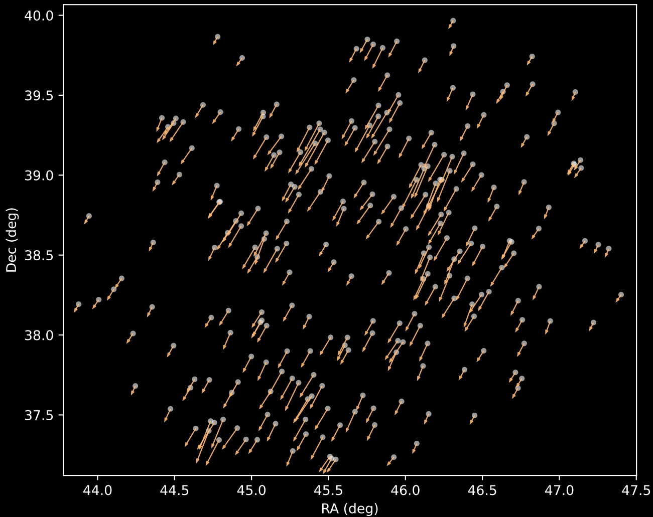
APOGEE DR17 Cluster 3 Proper Motion Vectors (n=246)
