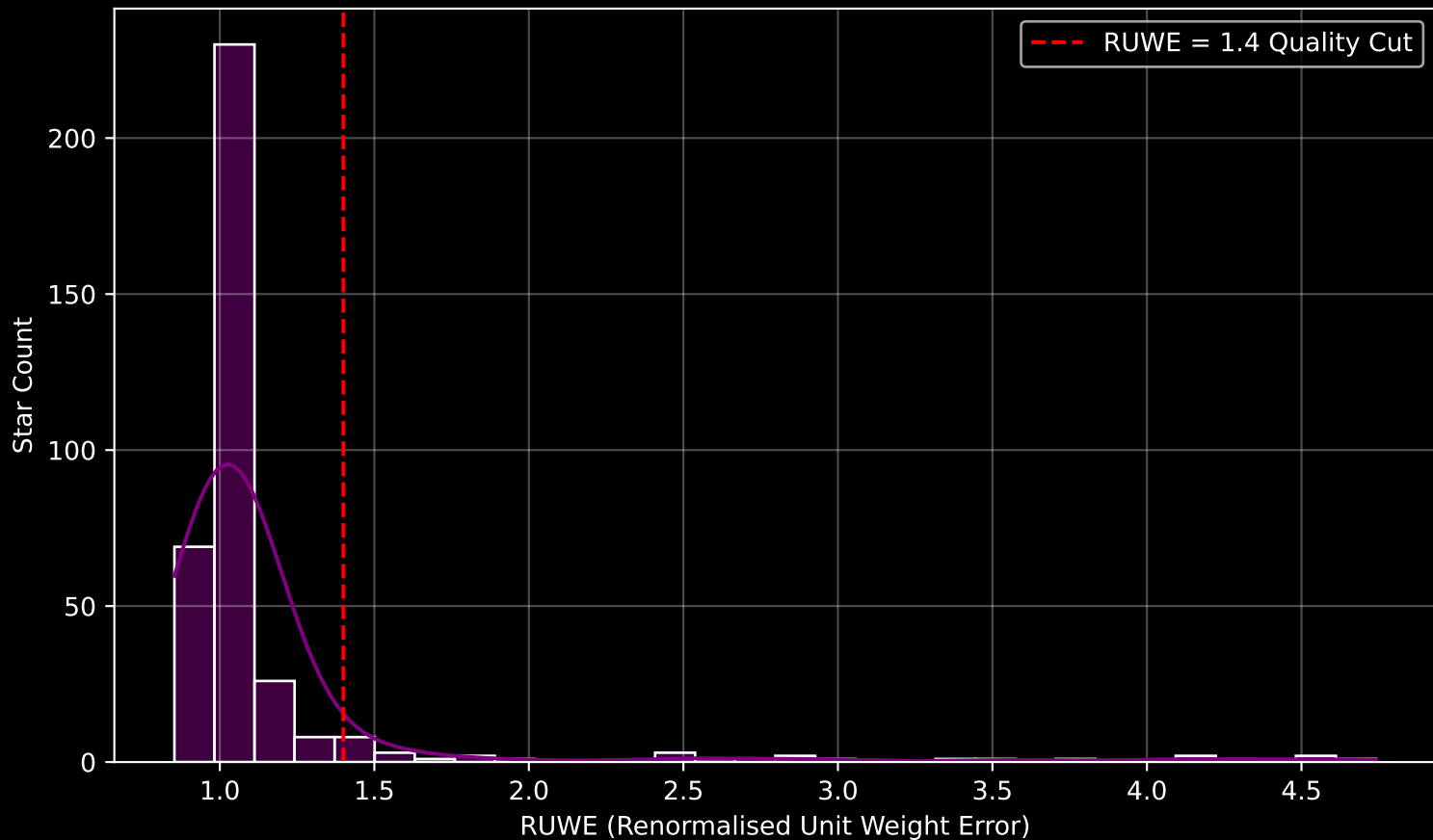
GAPOGEE DR17 Field [CygnusX_S_btx] RUWE Distribution (n= 364)
