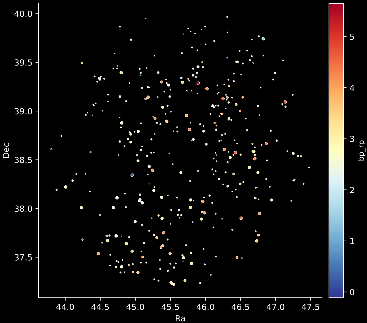
APOGEE DR17 Field: [CygnusX_S_btx] Stars: 372
