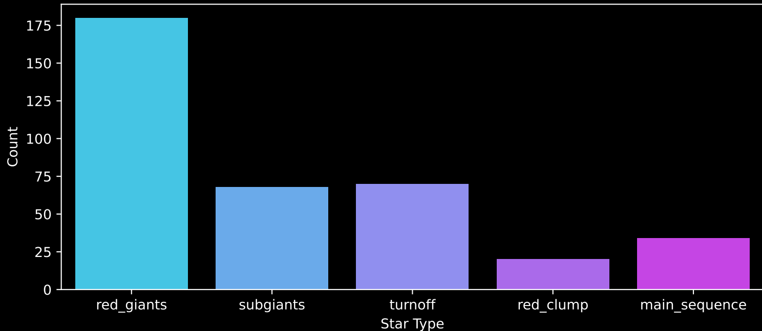
APOGEE DR17 Field: [CygnusX_S_btx] Count plot of Star Type
